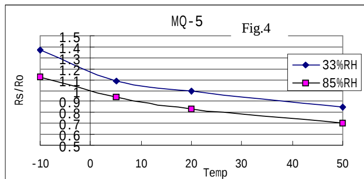
Fig.4 is shows the typical dependence of the MQ-5 on temperature and humidity. R_0 : sensor resistance at 1000ppm of H_2 in air at 33%RH and 20 degree.
